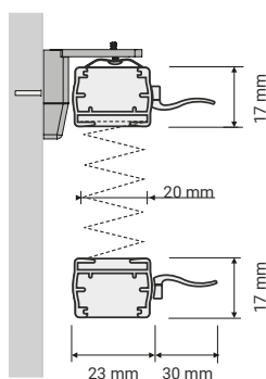
SIDE VIEW Wall mounting OPTIONAL
