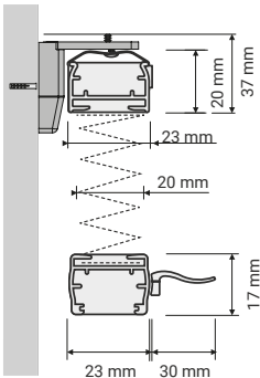
SIDE VIEW Wall mounting OPTIONAL
