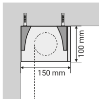
SIDE VIEW Wall mounting STANDARD
