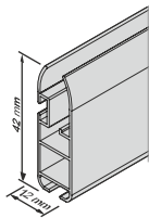
STANDARD END CAP Dimensions 12x42 mm
