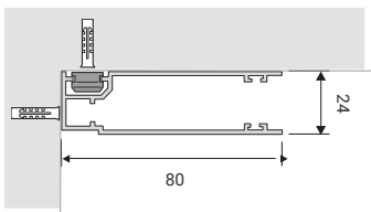
PROFILE SECTION Dimensions 80x24 mm
