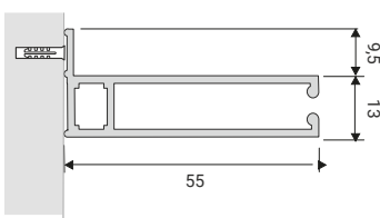
PROFILE SECTION Dimensions 55x22.5 mm
