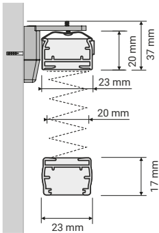
SIDE VIEW Wall mounting OPTIONAL
