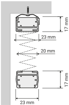
SIDE VIEW Ceiling mounting
