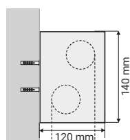
SIDE VIEW Wall fixing
