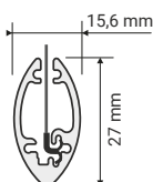
TEARDROP BOTTOM BAR Standard, with insert welded to the fabric.
