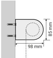
SIDE VIEW Wall fixing
