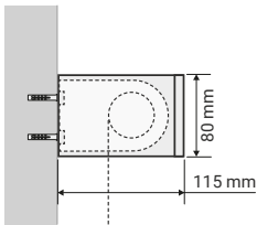
SIDE VIEW Wall fixing with main dimension and clearances.
