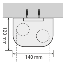
SIDE VIEW Ceiling fixing
