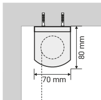
SIDE VIEW Ceiling fixing
