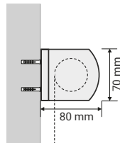
SIDE VIEW Wall fixing
