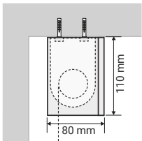
SIDE VIEW Ceiling fixing with main dimensions and clearances.
