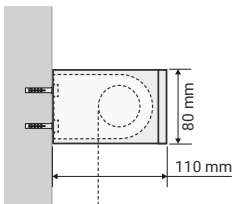
SIDE VIEW Wall fixing with main dimensions and clearances.
