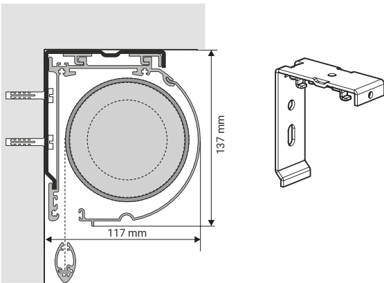
SIDE VIEW WITH WALL FIXING Ibox 114 with wall fixing
