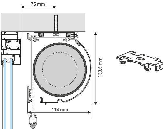
SIDE VIEW WITH CEILING FIXING Iibox 114 with ceiling fixing
