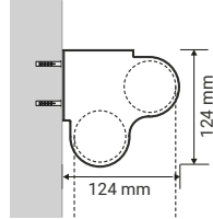
SIDE VIEW Wall fixing
