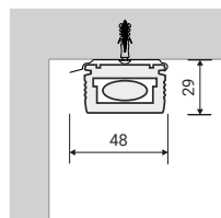
SIDE VIEW Ceiling mounting STANDARD
