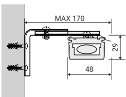
SIDE VIEW Wall mounting OPTIONAL
