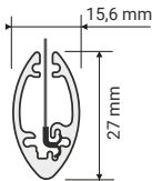
SIDE VIEW WITH WALL FIXING Ibox 90 with wall fixing
