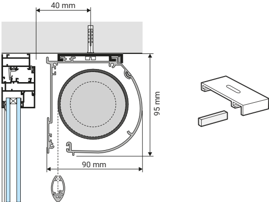
SIDE VIEW WITH CEILING FIXING Ibox 90 with ceiling fixing
