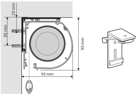
SIDE VIEW WITH WALL FIXING Ibox 90 with wall fixing
