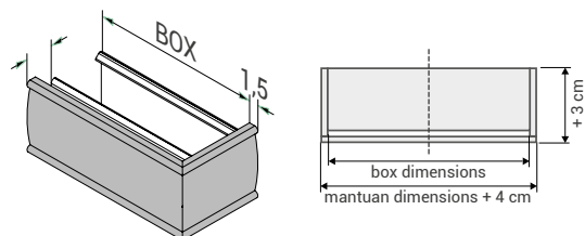
WOODEN MANTUAN AS STANDARD
