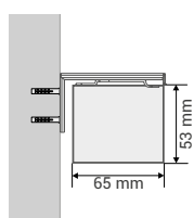
VIEW FROM THE SIDE Installation on wall
