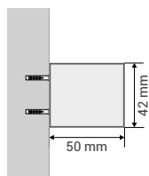
VIEW FROM THE SIDE Installation on wall
