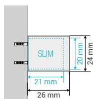
VIEW FROM THE SIDE Installation on wall
