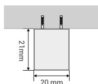
VIEW FROM THE SIDE Installation on ceiling
